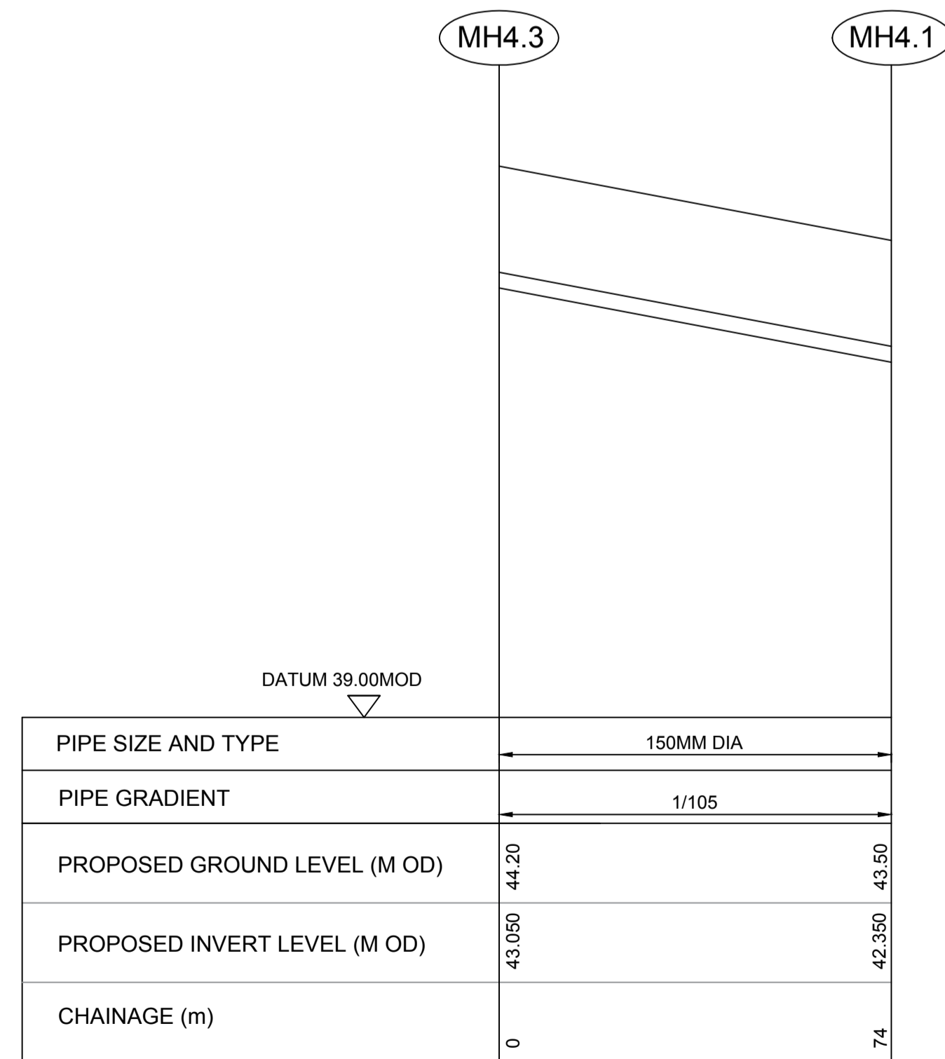
BIOMASS SLAB B: PIPE SECTION - MH4.3 TO MH4.1 SCALE: HORIZONTAL 1/1000, VERTICAL 1/50
