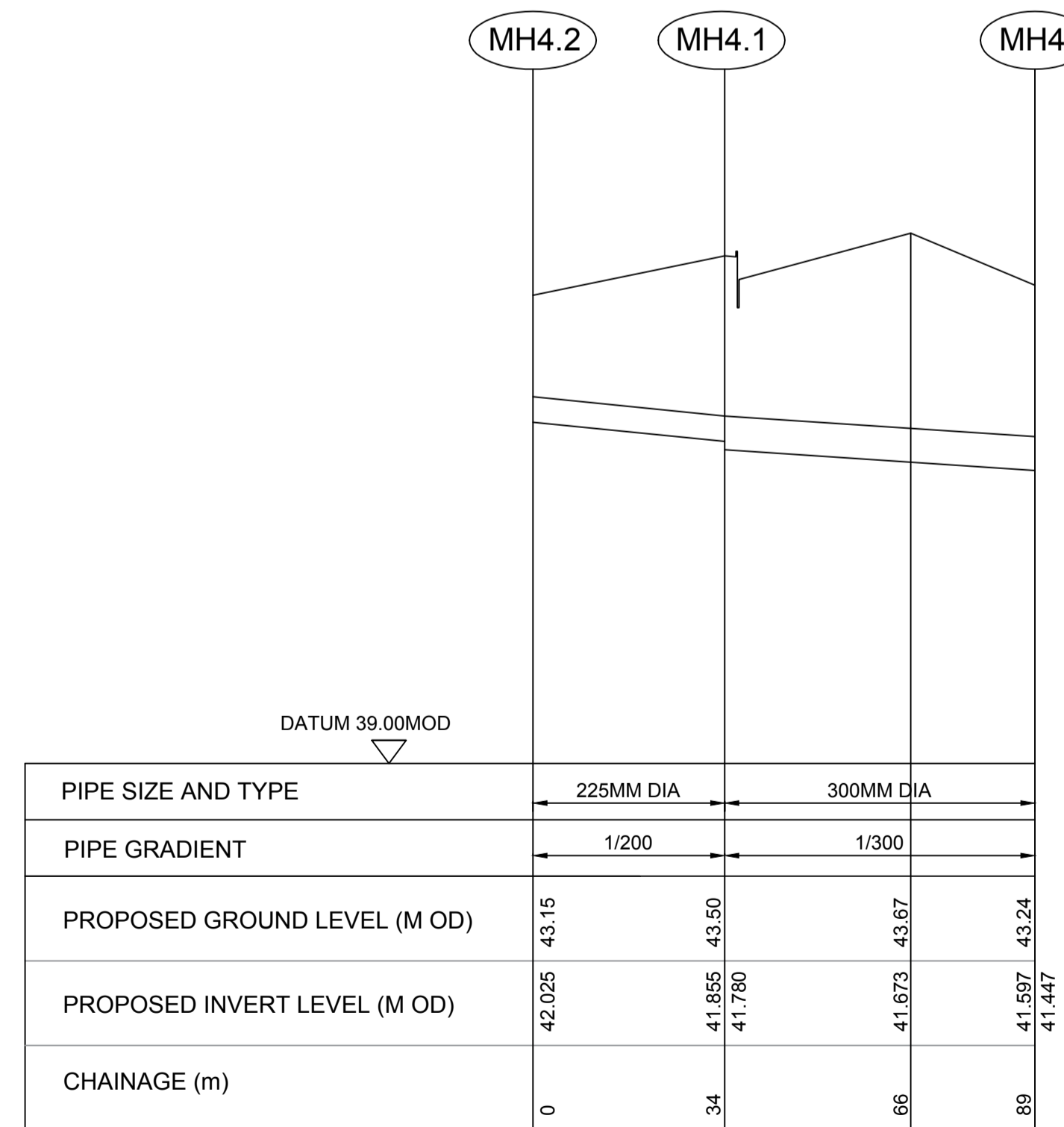
BIOMASS SLAB B: PIPE SECTION - MH4.2 TO MH4 SCALE: HORIZONTAL 1/1000, VERTICAL 1/50
