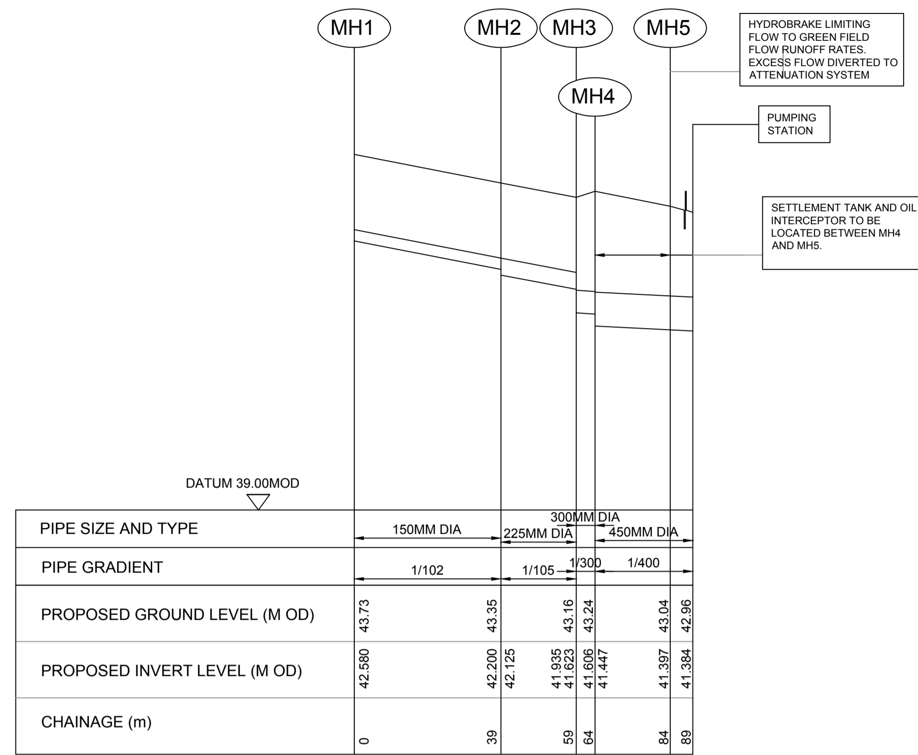
BIOMASS SLAB B: PIPE SECTION - CH 00 TO CH 89 (MH1 TO PUMPING STATION) SCALE: HORIZONTAL 1/1000, VERTICAL 1/50
